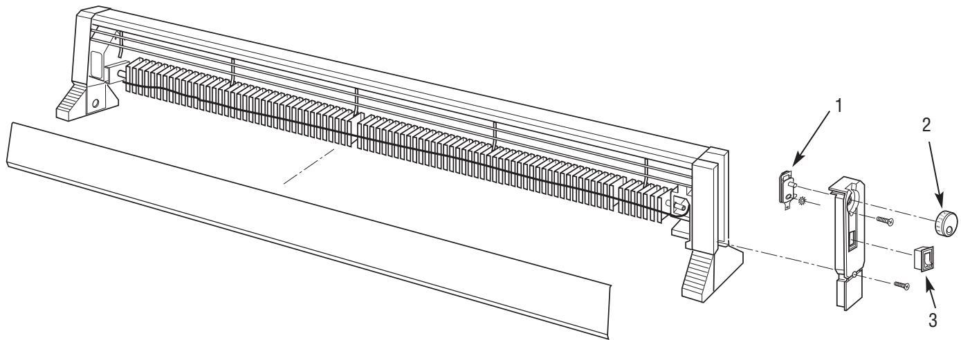
Figure 2 – Repair Parts
